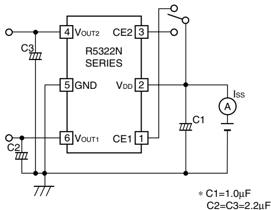
Fig.2 Supply Current Test Circuit
