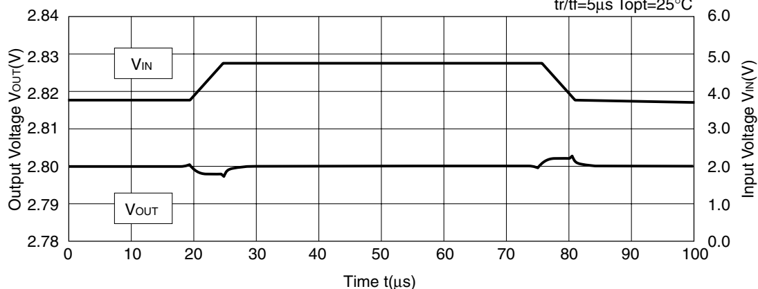
R5322N001× (2.8V, VR1)
